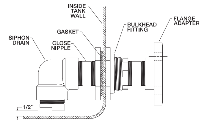
Bulkhead Fittings Available Sizes (Inches)
